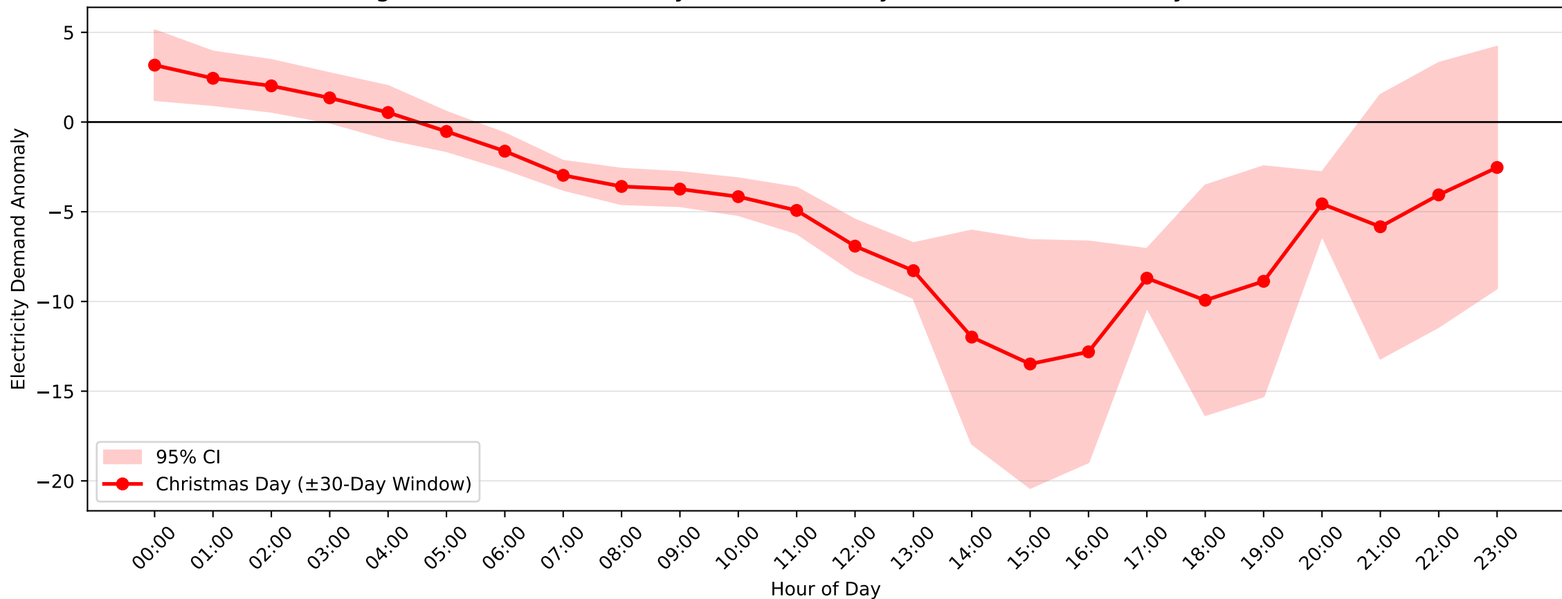
Kogarah Demand Anomaly: Christmas Day (2004–2017, \pm 30 -Day Window)
